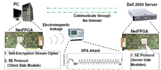
Figure 4. Prototype Implementation & Experiment Platform Construction.
